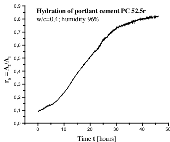
Figure 1: Portland cement paste modulus elasticity changes during the various stages of the hydration process.
