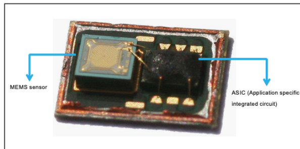
Figure 1: Example of MEMS microphone inside its package [6].
