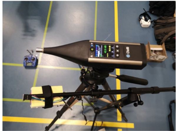
Figure 9: Validation experiment setup.
