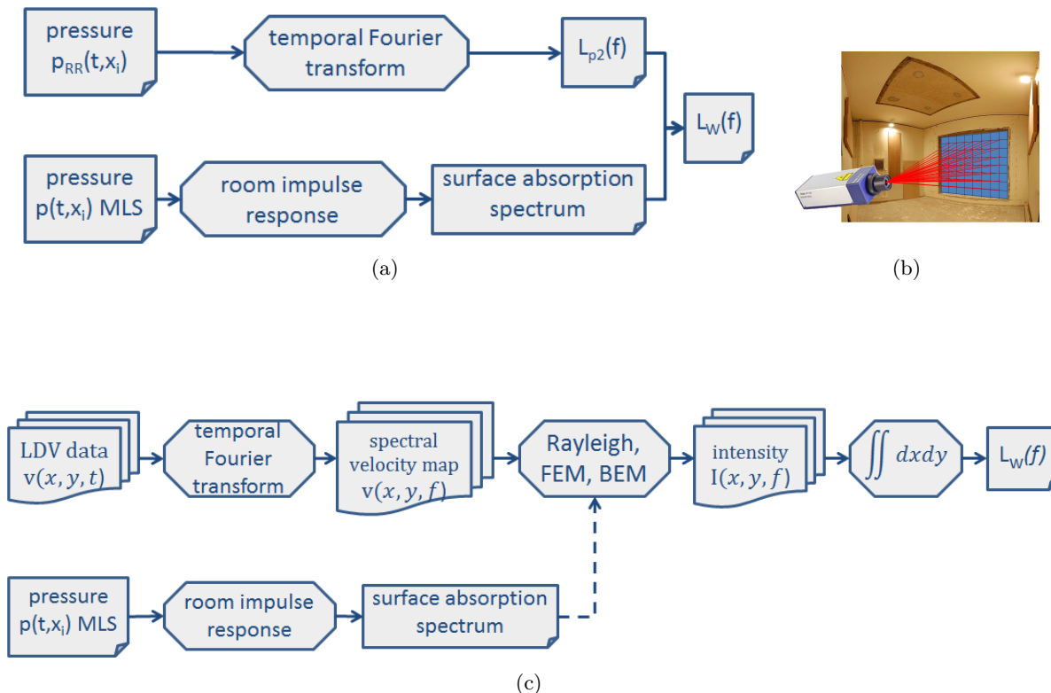
Figure 1: Methodologies to determine radiated sound power. (a) Microphone based ISO 10140. (b) Illustration of laser Doppler based approach (c) Laser Doppler based approach.
