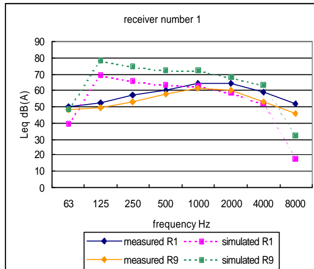
Figure 3. Comparison between measured and simulated LAeq values
