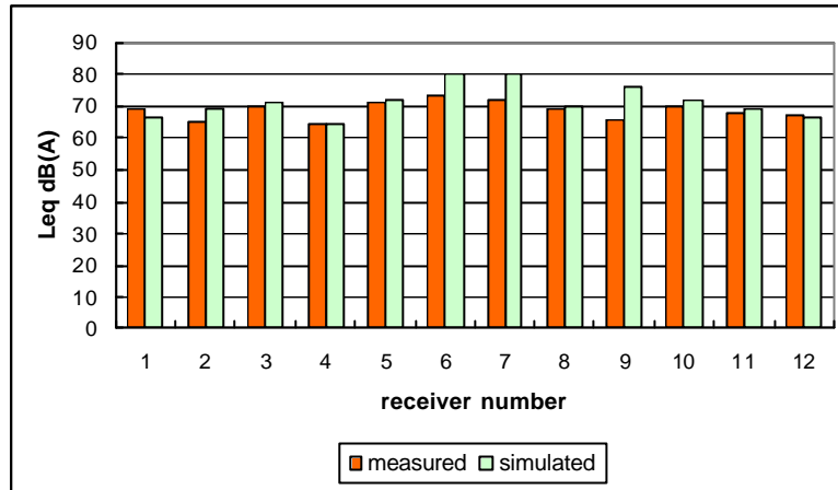
Figure 2. Comparison between measured and simulated LAeq values
