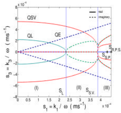
Fig. 7. Generalized slowness curves for (001)-[100] PZT4 layer.
