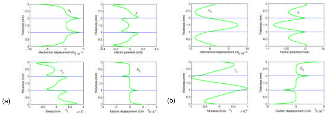
Fig. 5. Spatial distribution of fields in a (010)-[100] PZT5/(010)-[100] PZT5/(010)-[100] PZT5 short-circuited piezoelectric sandwich structure: (a) f_{xh}=17.9 \text{ MHz} and v_{ph}=2.11 \text{ mm.}10^6 \text{ s}^{-1} ; (b) f_{xh}=17.9 \text{ MHz} and v_{ph}=2.47 \text{ mm.}10^6 \text{ s}^{-1} .
