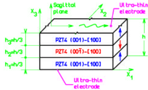
Fig. 2. Infinite piezoelectric sandwich plate in PZT4: geometry and notations.
