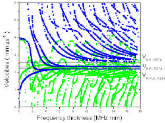
Fig. 6. Dispersion curves for Lamb waves in a (001)-[100] PZT4/(001)-[100] PZT4/(001)-[100] PZT4 short-circuited piezoelectric sandwich plate.
