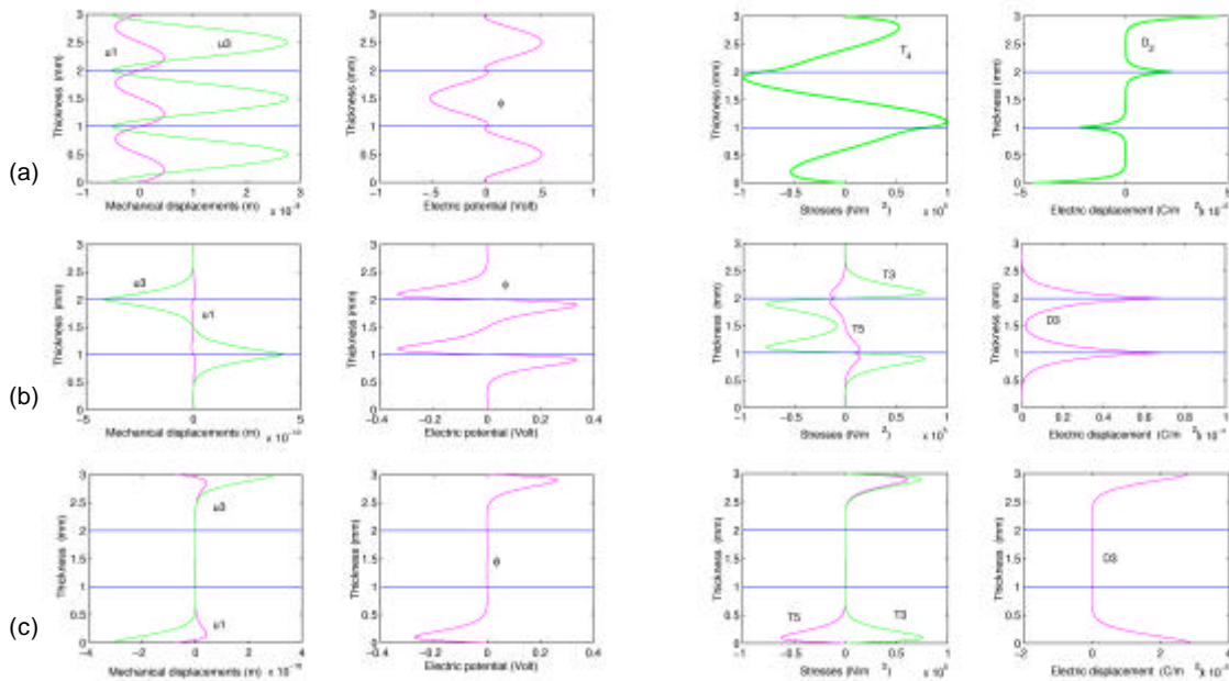
Fig. 8. Spatial distribution of fields in a (001)-[100] PZT4/(001)-[100] PZT4/(001)-[100] PZT4 short-circuited piezoelectric sandwich structure: (a) f_{xh}=17.09 \text{ MHz} and v_{S.V. PZT4}=2.62 \text{ mm.10}^6 \text{ s}^{-1} ; (b) f_{xh}=15.5 \text{ MHz} and v_{S.P. PZT4}=2.47 \text{ mm.10}^6 \text{ s}^{-1} ; (c) f_{xh}=14.25 \text{ MHz} and v_{R.P.S. PZT4}=2.47 \text{ mm.10}^6 \text{ s}^{-1} .
