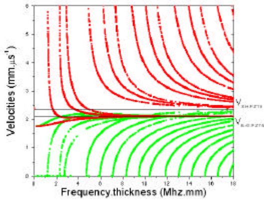
Fig. 3. Dispersion curves for SH waves in a (010)-[100] PZT5/(010)-[100] PZT5/(010)-[100] PZT5 short-circuited piezoelectric sandwich plate.
