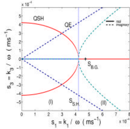
Fig. 4. Generalised slowness curves for (010)-[100] PZT5 layer.
