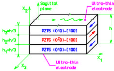
Fig. 1. Infinite piezoelectric sandwich plate in PZT5: geometry and notations.
